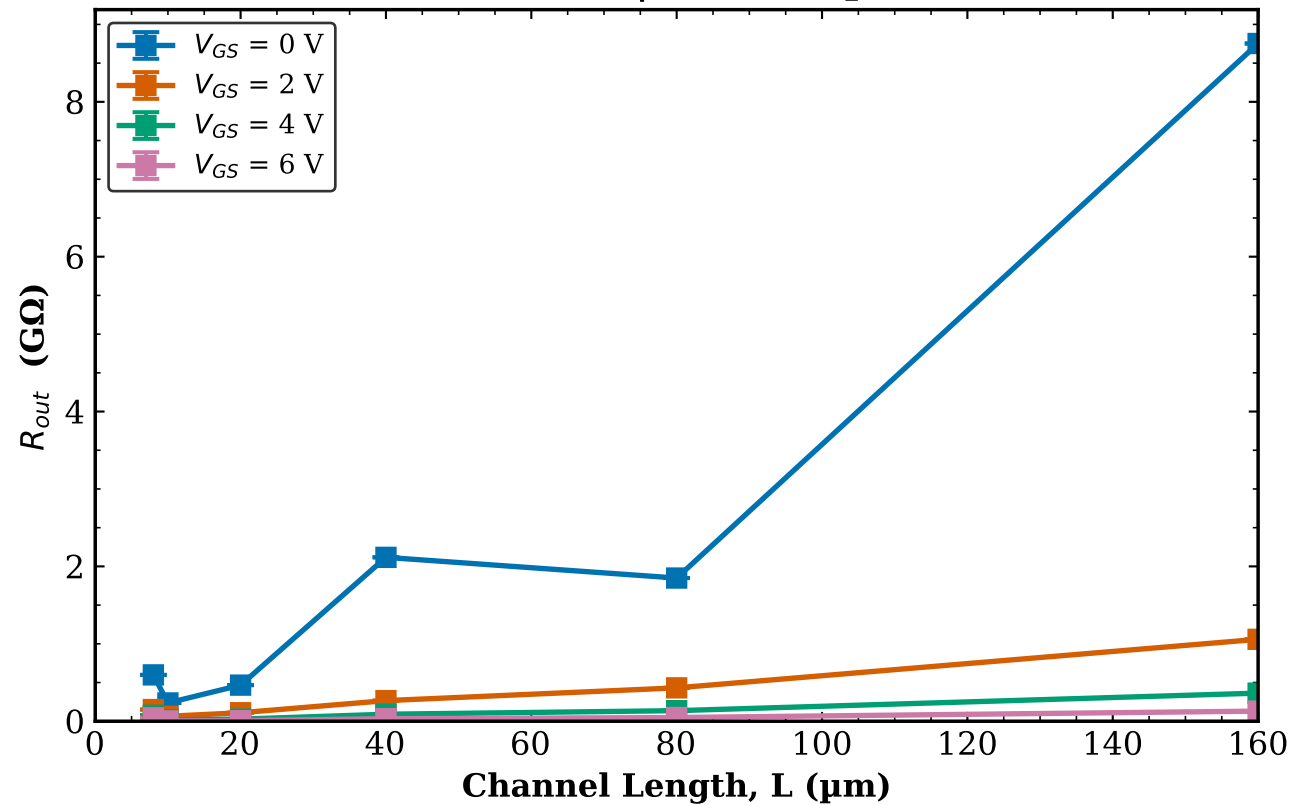
TFT1 Transistor 1 R_{out} vs L | W = 10 \mu\text{m}
